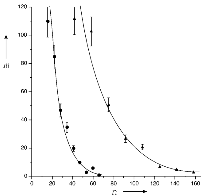
Figure 2. Experimental length distribution of PAC-1 ( \Delta ) and PAC-2 ( \bullet ) determined by SFM and calculated length distribution (—) based on binding energies of 21.5 k_B T ( 53.4 \text{ kJ mol}^{-1} , PAC-1) and 19 k_B T ( 47.2 \text{ kJ mol}^{-1} , PAC-2). n = number of repeat units, m = occurrence.
